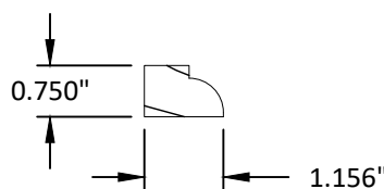
GLASS STOP WJ PROFILE - WOOD
