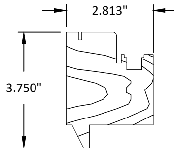
TOP RAIL WH (IG) PROFILE - WOOD
