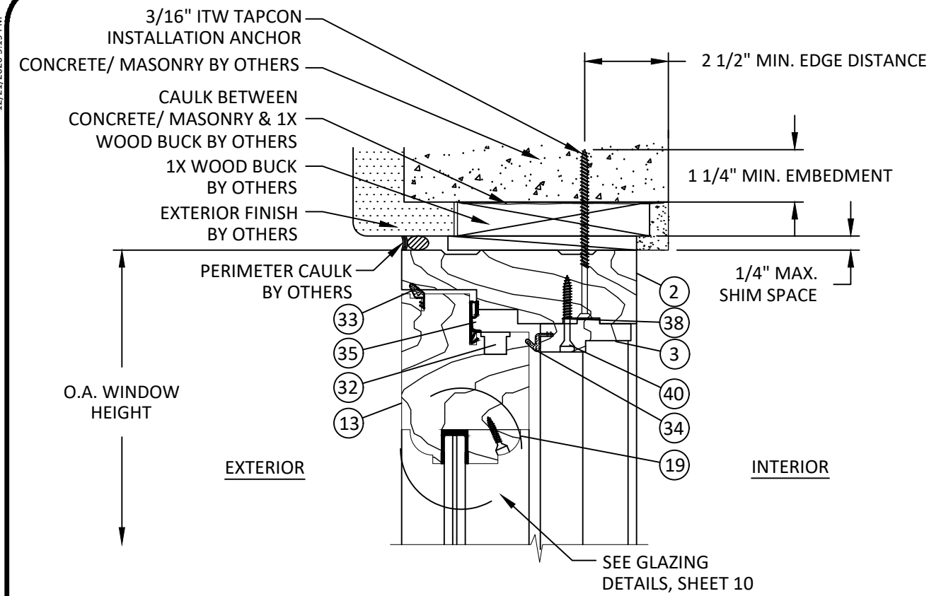
F 5 VERTICAL SECTION HEAD - CONCRETE/MASONRY WJ SASH PROFILE
