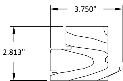
STILE HINGE SIDE WH (IG) PROFILE - WOOD
