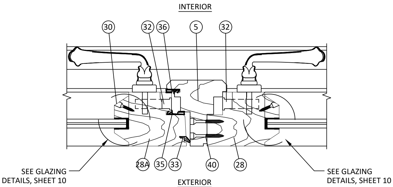
P 7 HORIZONTAL SECTION ASTRAGAL WH (MONO) SASH PROFILE
