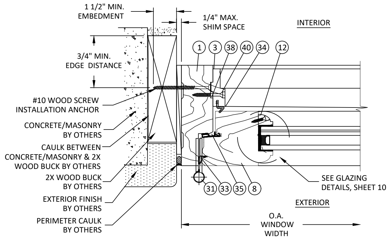
C 4 HORIZONTAL SECTION JAMB - 2X WOOD BUCK WI SASH PROFILE
