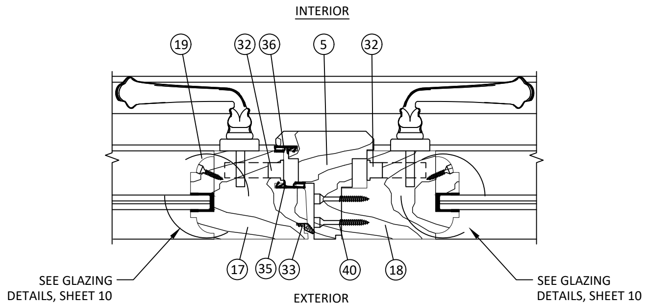
H 5 HORIZONTAL SECTION ASTRAGAL WJ SASH PROFILE
