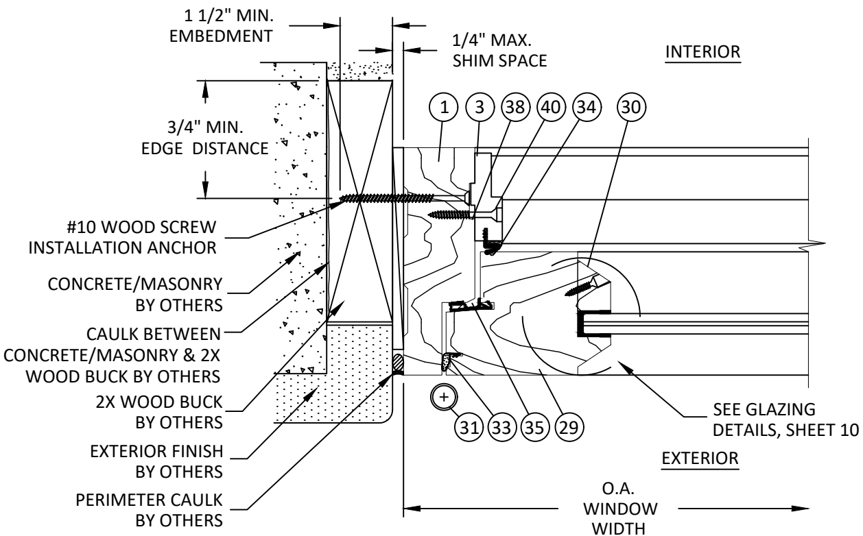
O 7 HORIZONTAL SECTION JAMB - 2X WOOD BUCK WH (MONO) SASH PROFILE
