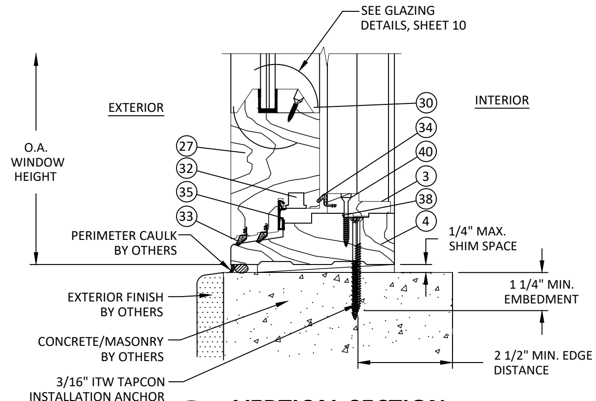
M 7 VERTICAL SECTION SILL - CONCRETE/MASONRY WH (MONO) SASH PROFILE
