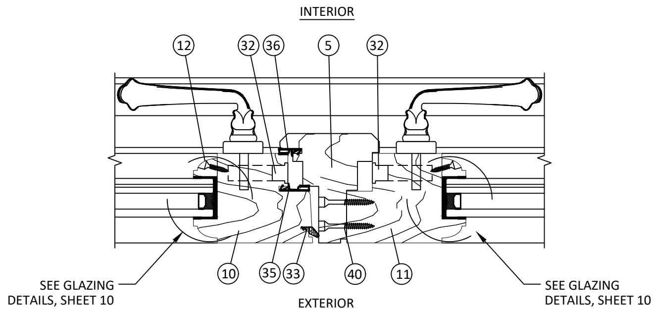
D 4 HORIZONTAL SECTION ASTRAGAL WI SASH PROFILE
