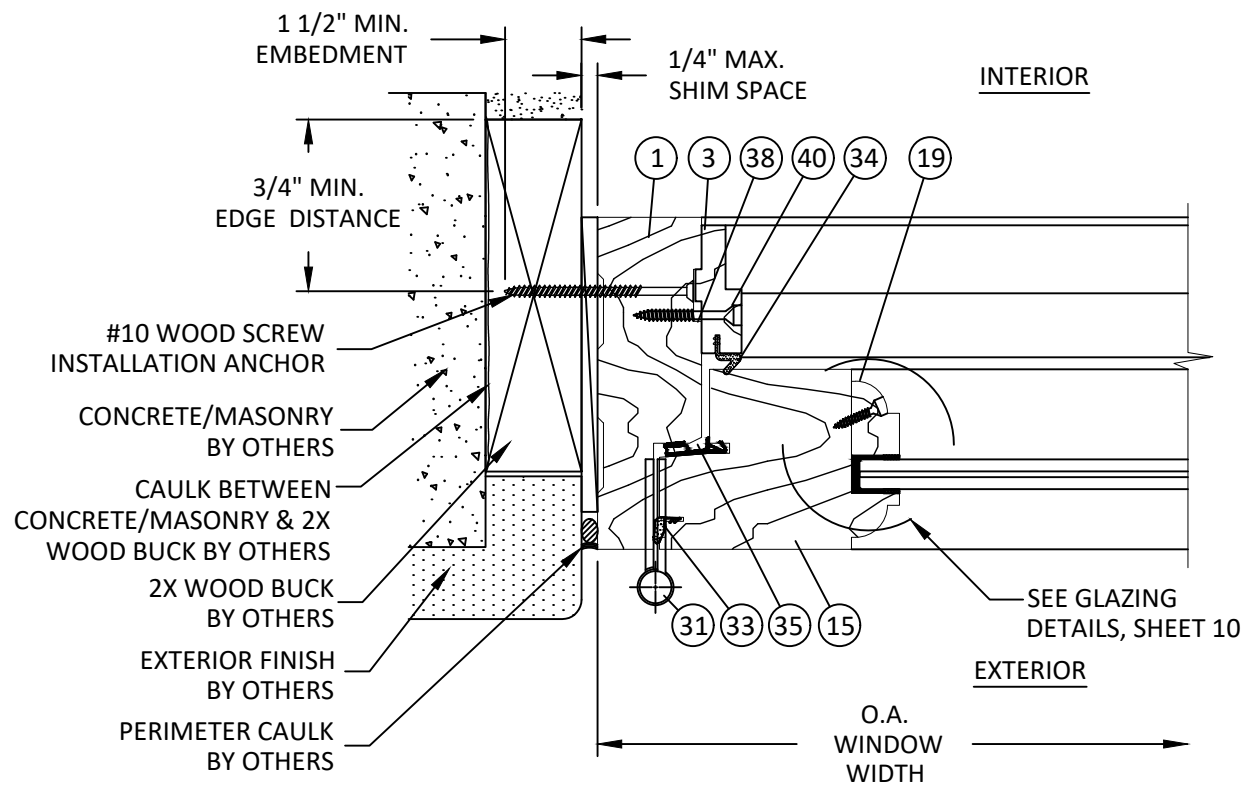
G 5 HORIZONTAL SECTION JAMB - 2X WOOD BUCK WJ SASH PROFILE
