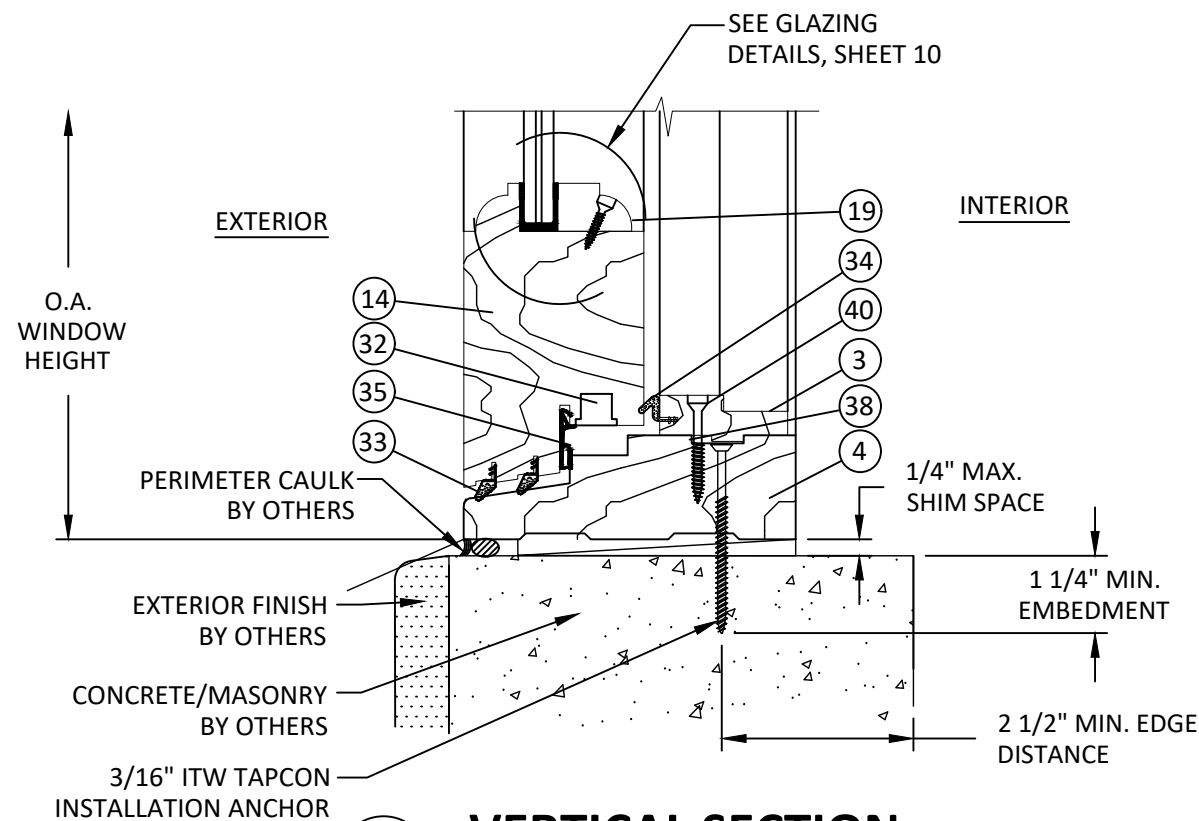
E 5 VERTICAL SECTION SILL - CONCRETE/MASONRY WJ SASH PROFILE
