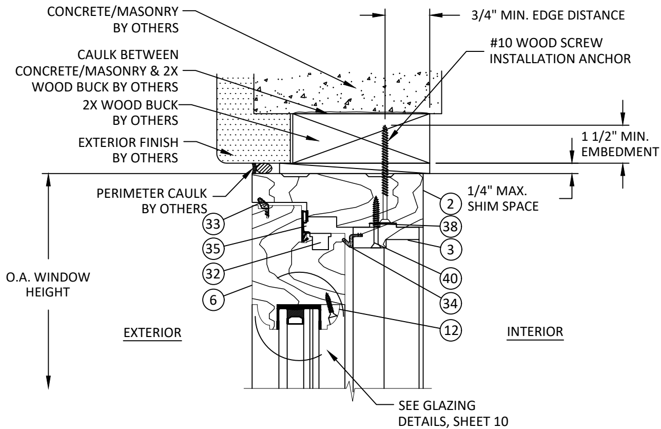
B 4 VERTICAL SECTION HEAD - 2X WOOD BUCK WI SASH PROFILE
