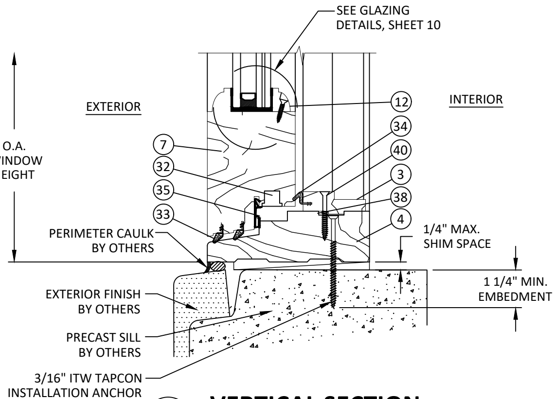
A 4 VERTICAL SECTION SILL - CONCRETE/MASONRY PRE-CAST SILL - WI SASH PROFILE
